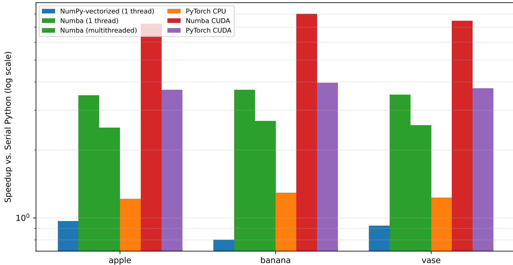
Speedup at N=5000 (Colab, float32)
